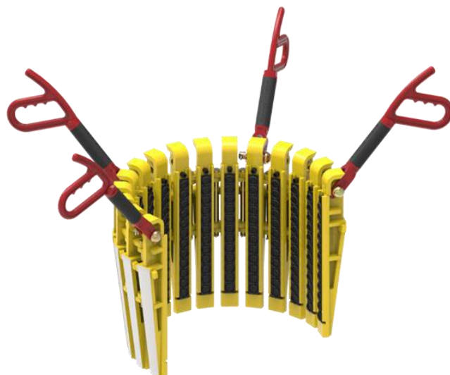
KET “CMS-3” CASING SLIPS COMPLETE
